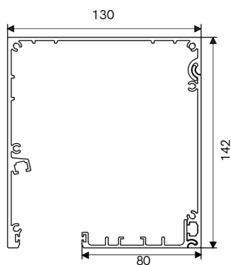
KASSETT 130 COMPACT
