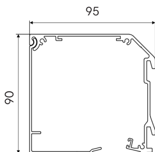
KASSETT 90
